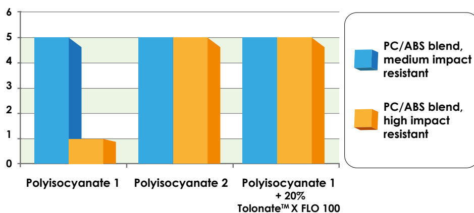
Graph 3 : Improvement of direct to plastic adhesion thanks to Tolonate™ X FLO 100 Crosshatch adhesion test after 3 days in hot water (40°C) / 5 = good / 0 = fail
