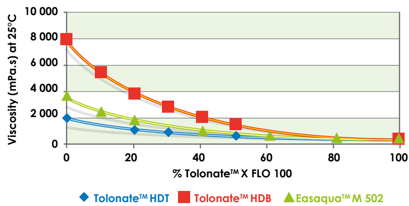
Graph 1: Effect of Tolonate™ X FLO 100 on the viscosity
