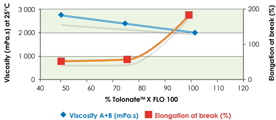
Graph 4: Benefit of Tolonate™ X FLO 100 (blended with HDI trimer)
