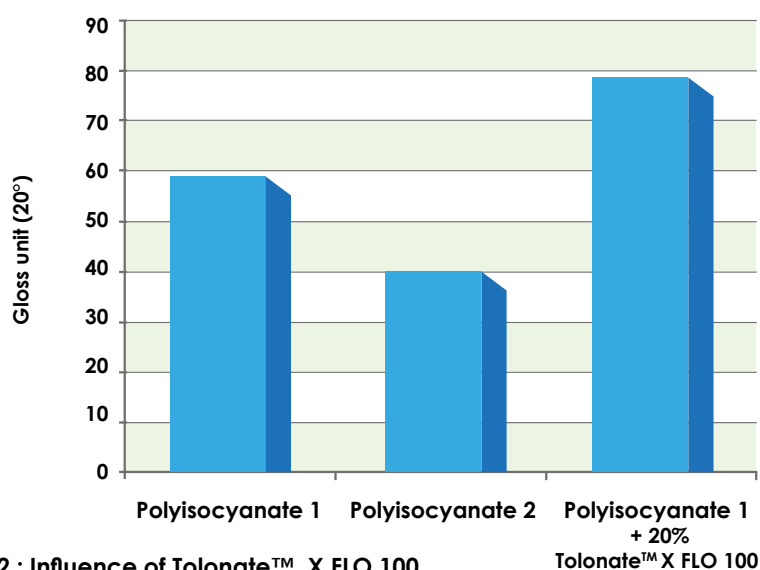
Graph 2 : Influence of Tolonate™ X FLO 100 on the gloss of coated plastic substrates
