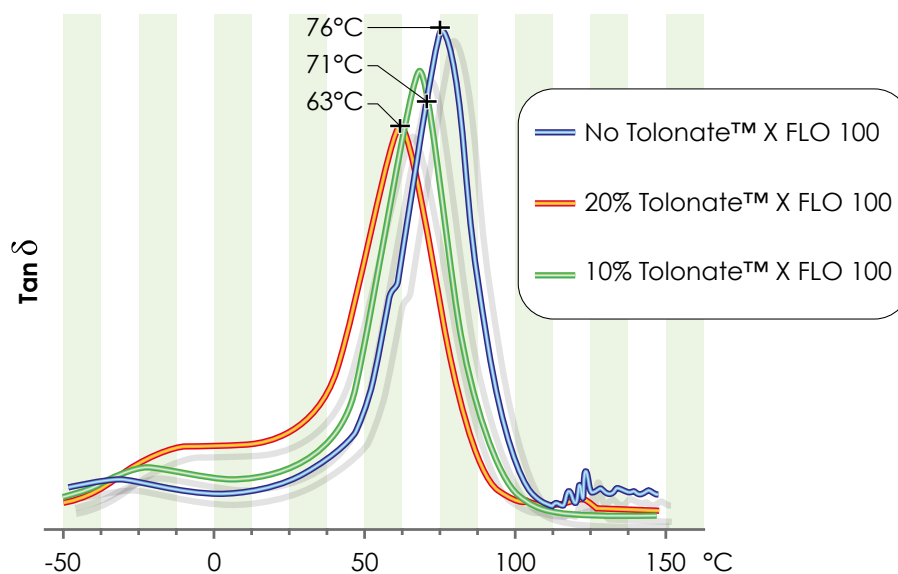
Graph 5: Effect of Tolonate™ X FLO 100 on Tg
